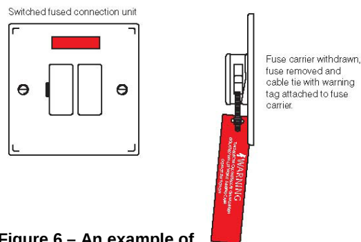
Figure 6 – An example of securing a fuse carrier
