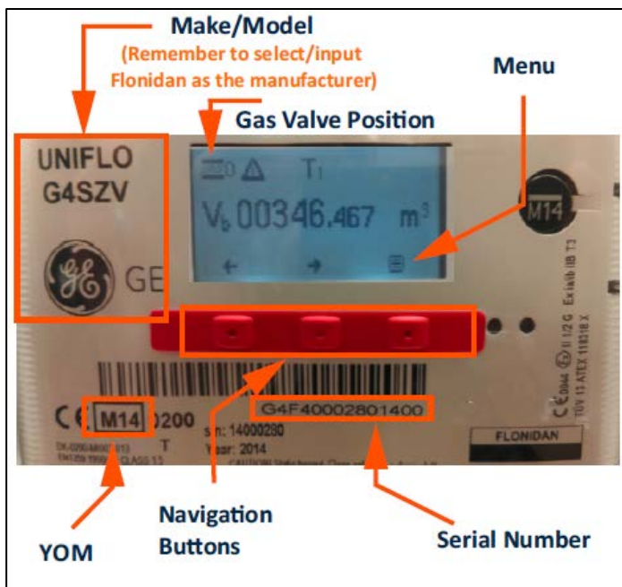
Figure 2 shows the smart module which is fitted to the Flonidan Smart meter
